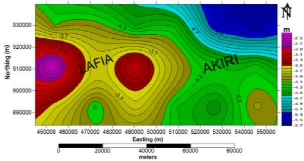
Figure 9. Deep depth to basement map.
