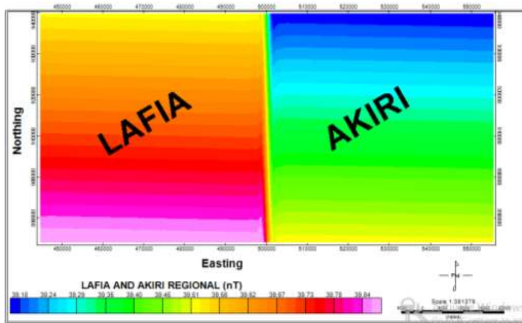
Figure 5. Regional magnetic intensity (TMI) map of the study area.
