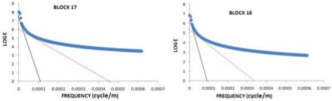
Figure 8. Spectral plots of logarithm of Energy against Frequency (cycle per meter).
