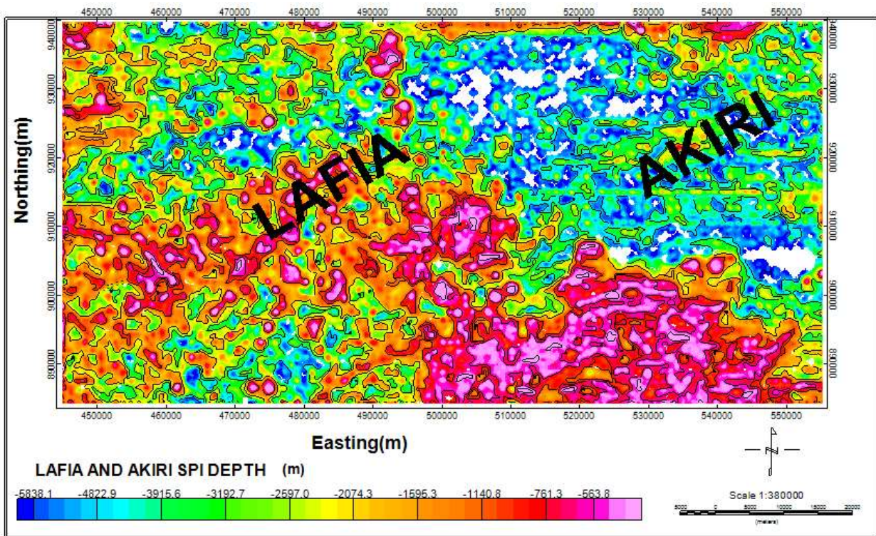
Figure 12. Source parameter image (SPI) map of the study area.
