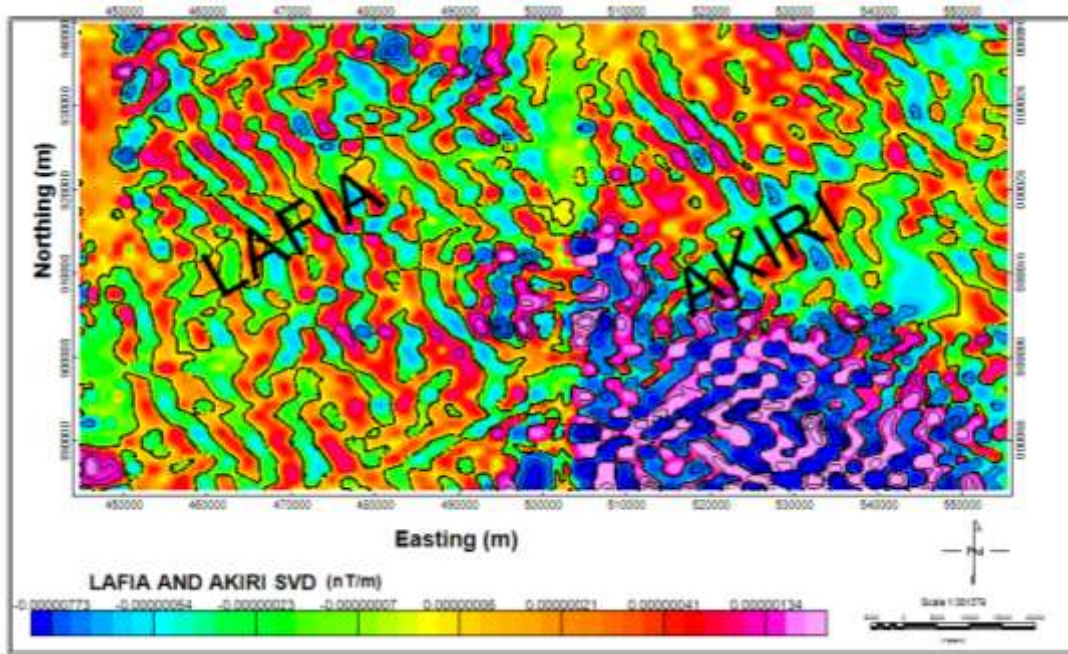
Figure 4. SVD map of the study area.
