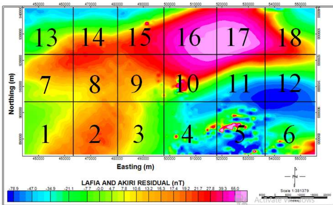
Figure 7. Division into 18 spectral blocks for estimation of the depth to basement.
