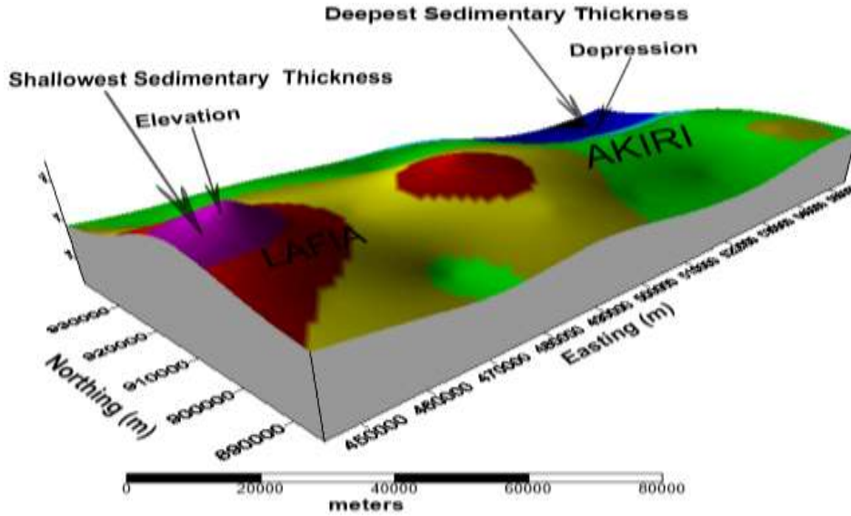
Figure 11. 3D map of the study area showing magnetic basement topography.
