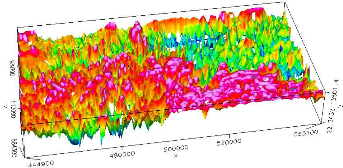
Figure 13. The 3-D SPI view of the study area.
