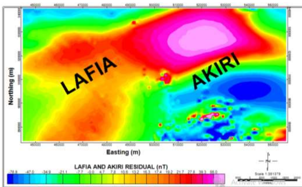
Figure 6. The residual magnetic intensity (TMI) map of the study area.
