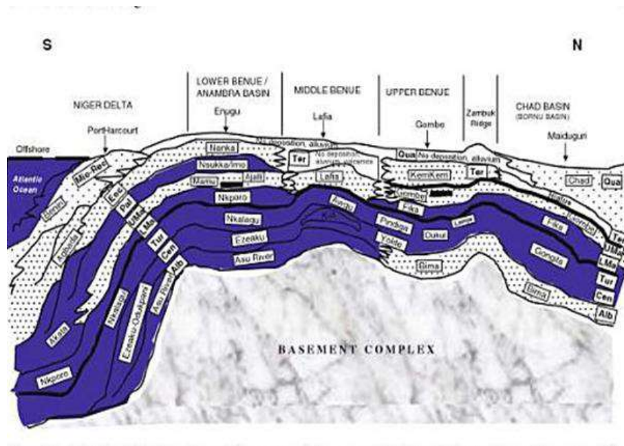
Figure 1b. Stratigraphic succession in the Benue trough (Obaje, 2004).
